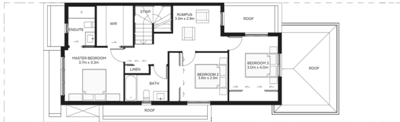
FIRST FLOOR
